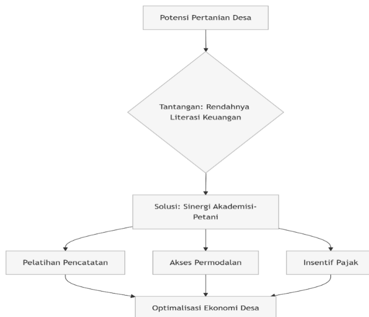
Gambar 1 Flowchart Pengabdian
