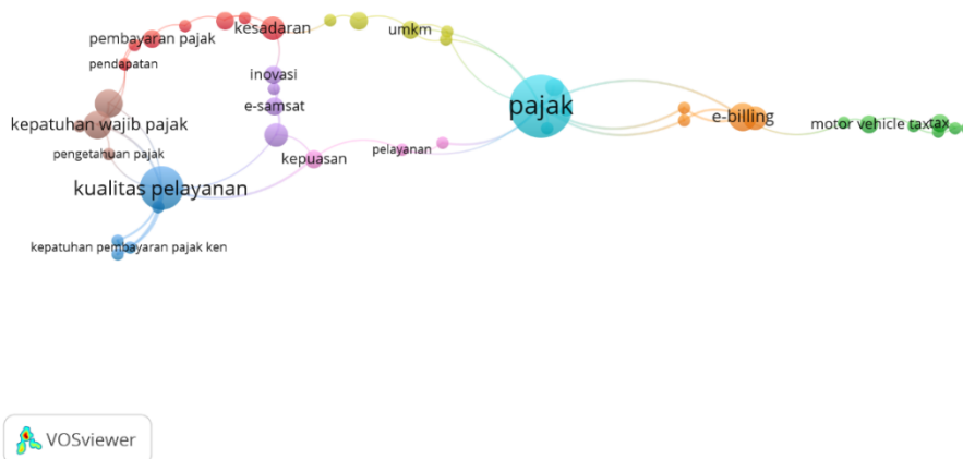
Gambar 1 : Network Visualization
