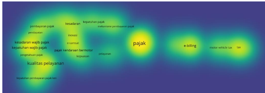
Gambar 3 : Density Visualization
